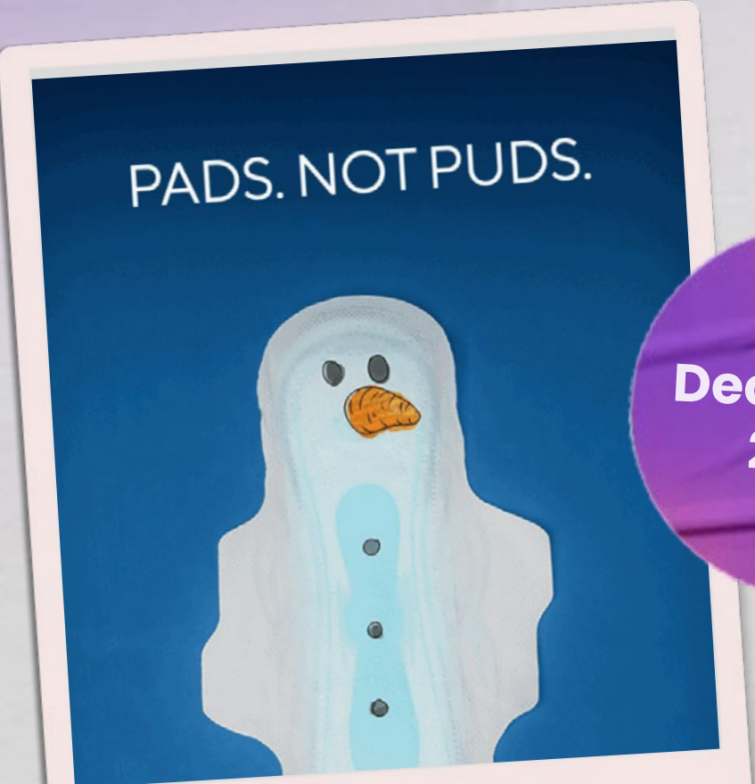
AML group
