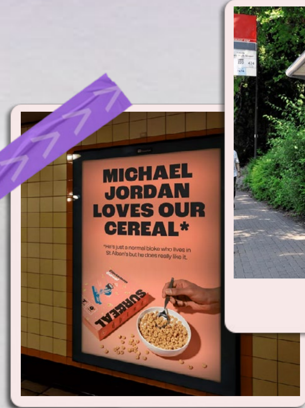
Surreal
