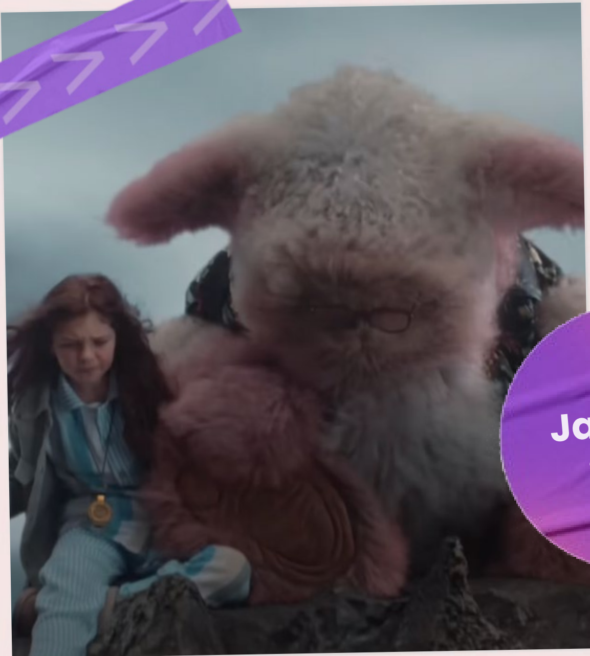
Apple
